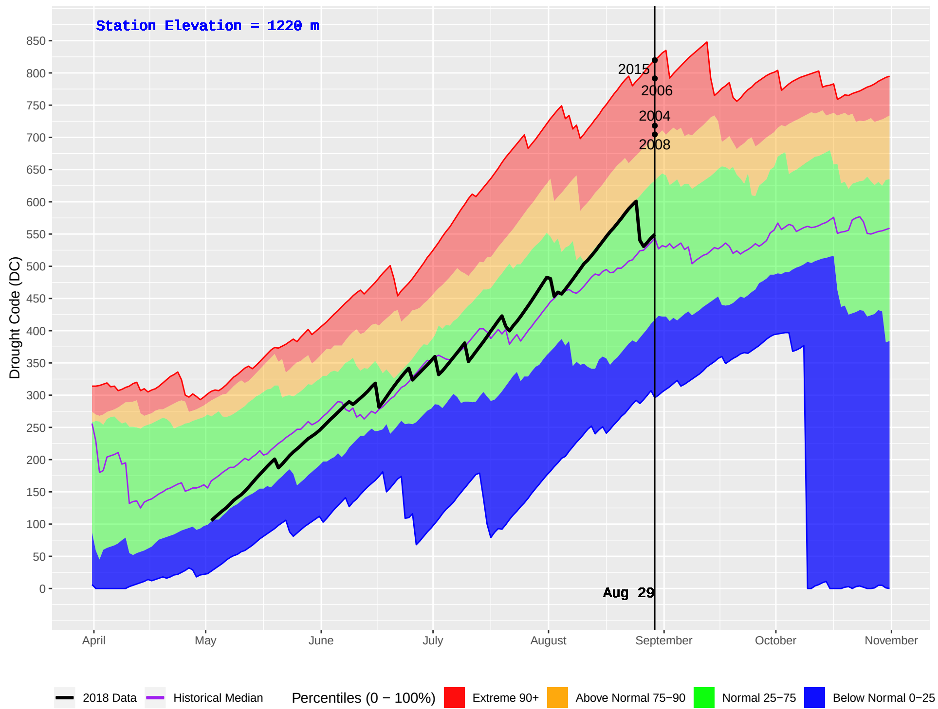
NEMIAH (216) : Historical (1982–2016) and Current (2018) Daily Drought Code (DC)
