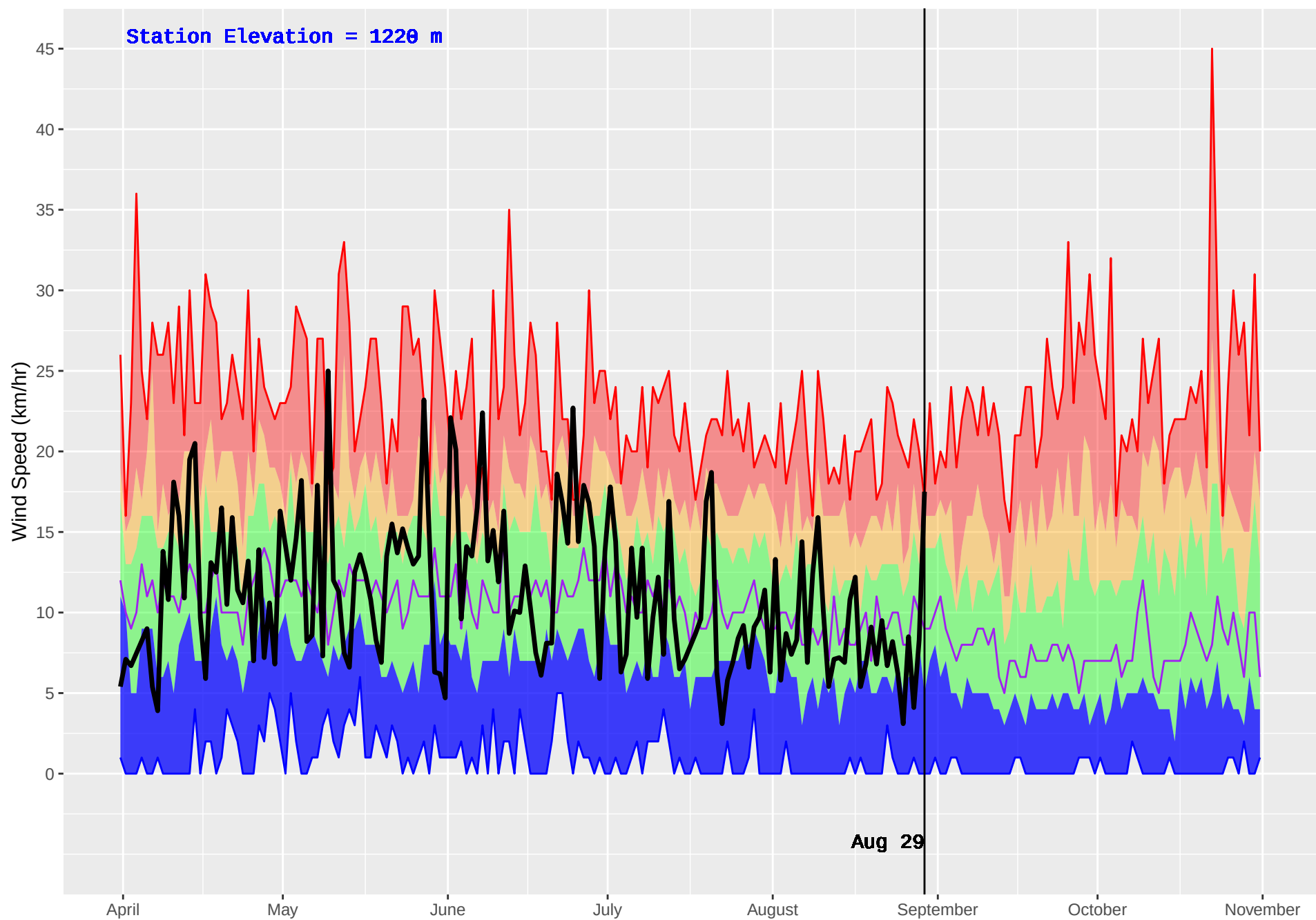
NEMIAH (216) : Historical (1982–2016) and Current (2018) Daily Wind Speed
