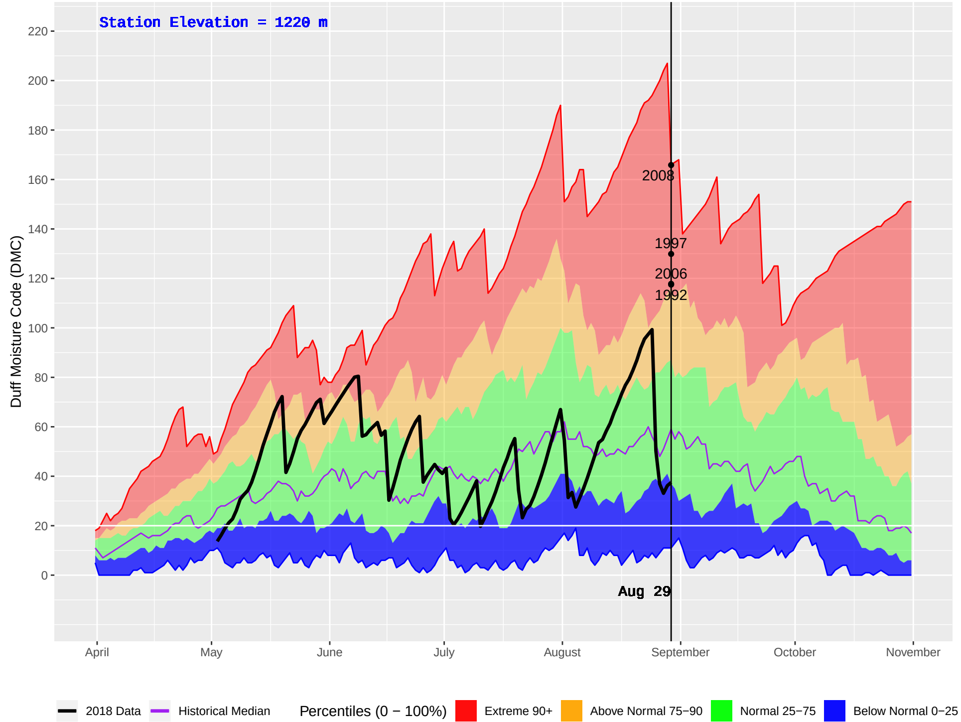
NEMIAH (216) : Historical (1982–2016) and Current (2018) Daily Duff Moisture Code (DMC)
