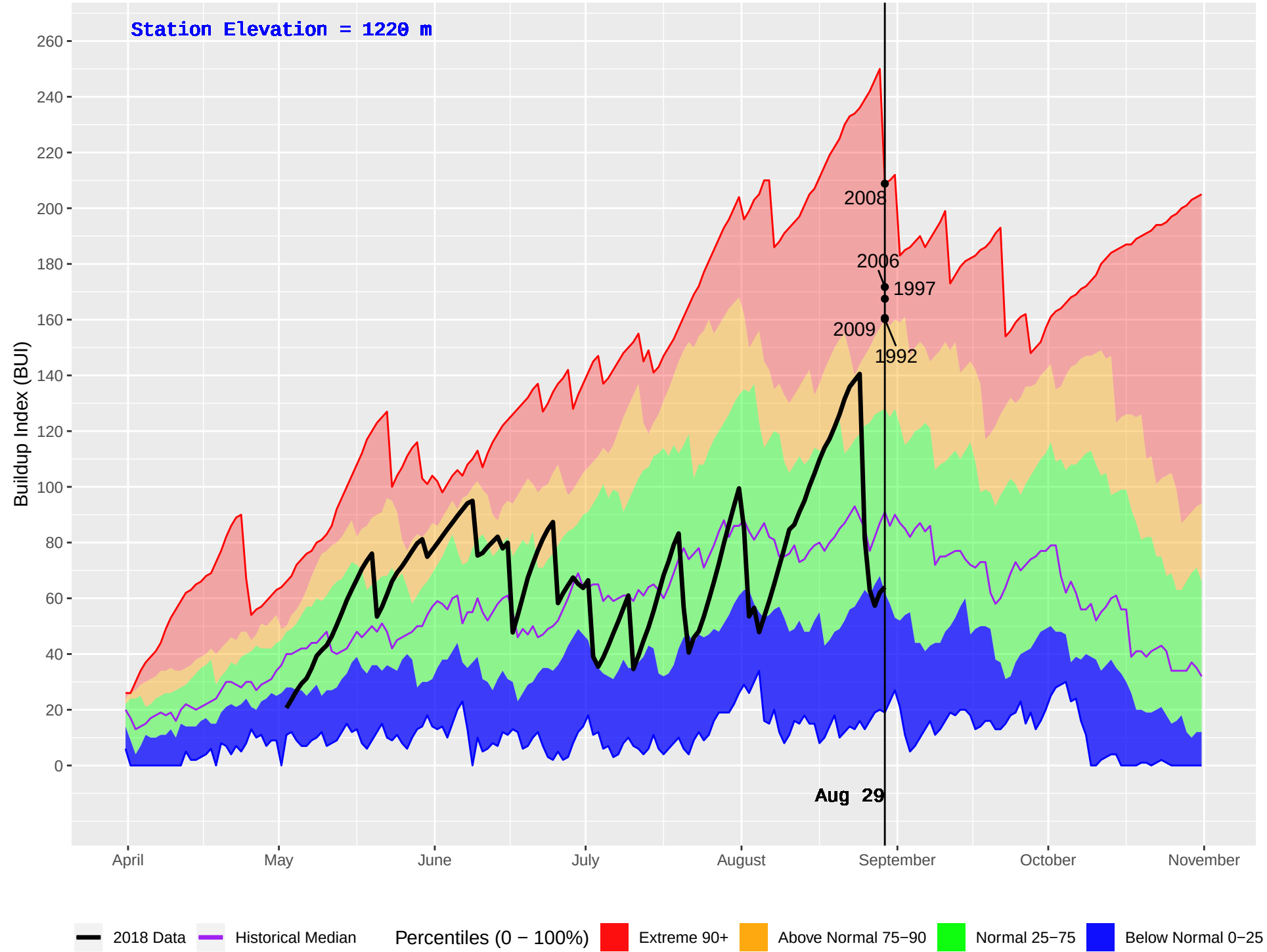
NEMIAH (216) : Historical (1982–2016) and Current (2018) Daily Buildup Index (BUI)
