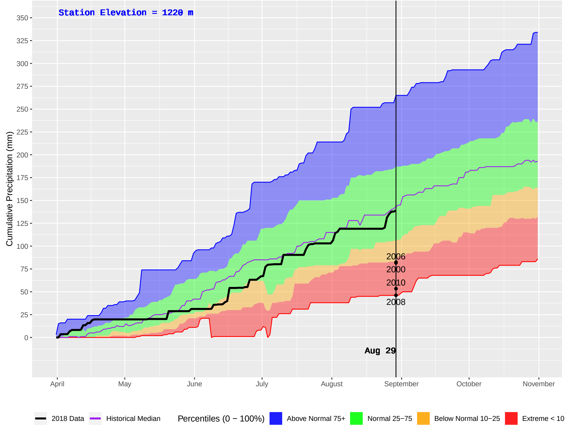
NEMIAH (216) : Historical (1982–2016) and Current (2018) Daily Cumulative Precipitation
