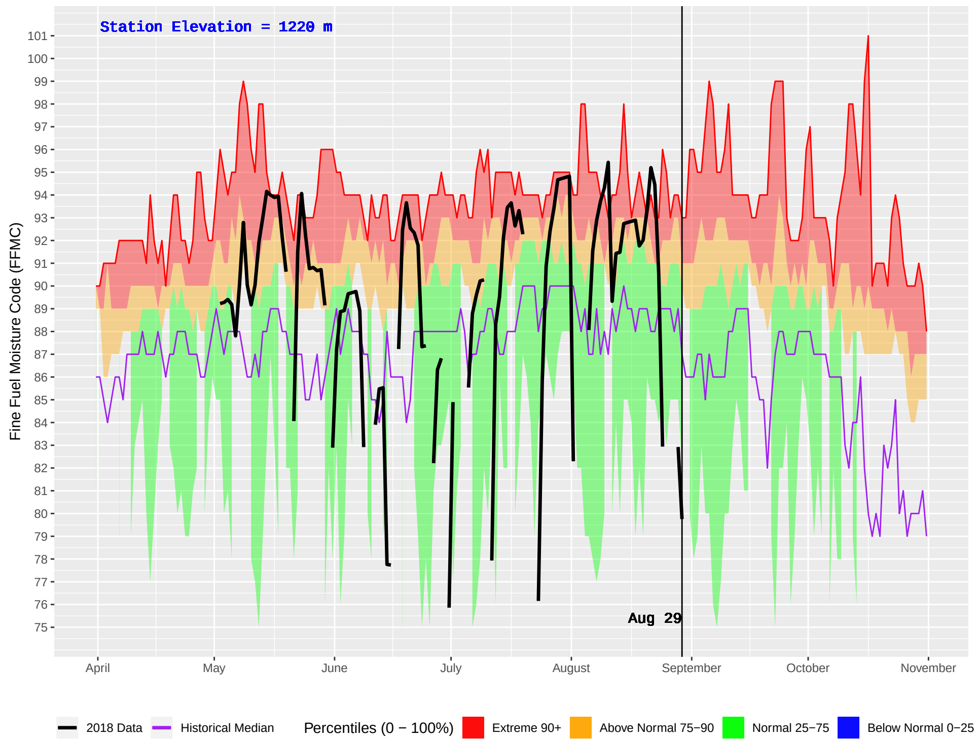
NEMIAH (216) : Historical (1982–2016) and Current (2018) Daily Fine Fuel Moisture Code (FFMC)
