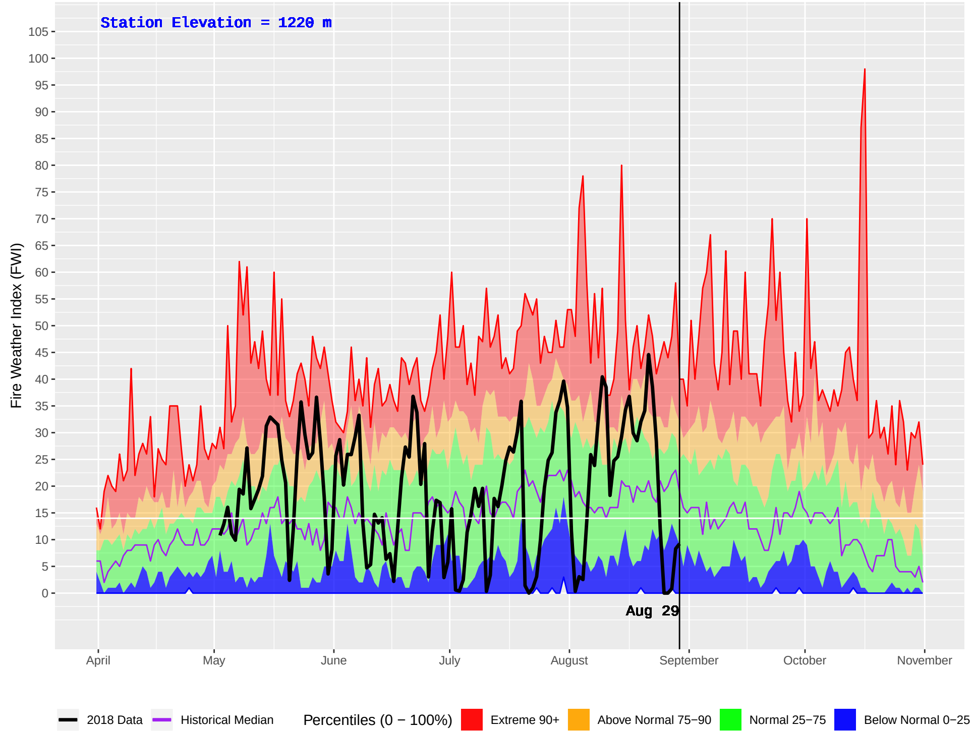
NEMIAH (216) : Historical (1982–2016) and Current (2018) Daily Fire Weather Index (FWI)
