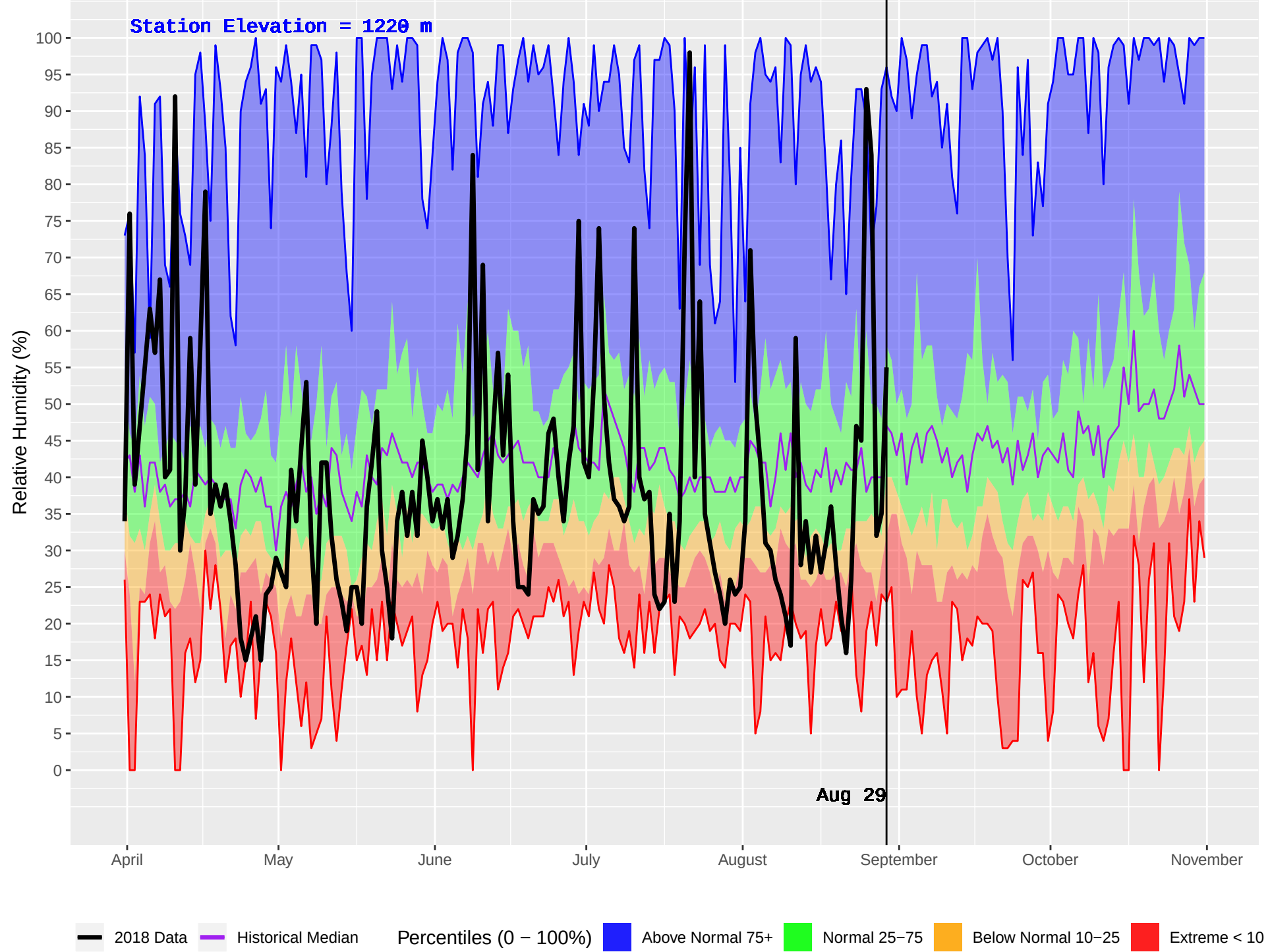
NEMIAH (216) : Historical (1982–2016) and Current (2018) Daily Relative Humidity
